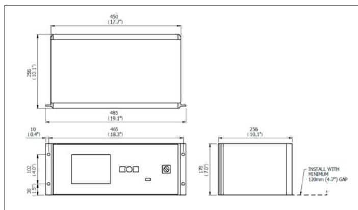
Optional Condumax II Remote Interface
